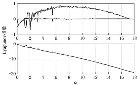
图 2 Lyapunov 指数谱, \beta = 20, \gamma = 0.01, a = -3, b = 1, \alpha \in [0, 18]
