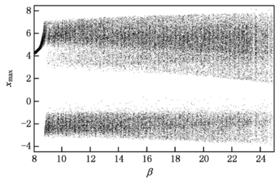
图 5 分岔图, \alpha = 6, \gamma = 0.01, a = -3, b = 1, \beta \in [8, 25]
