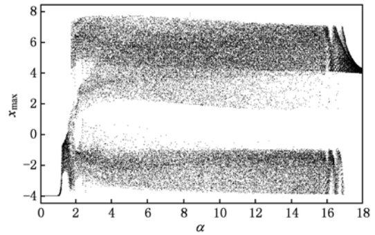
图 3 分岔图, \beta = 20, \gamma = 0.01, a = -3, b = 1, \alpha \in [0, 18]
