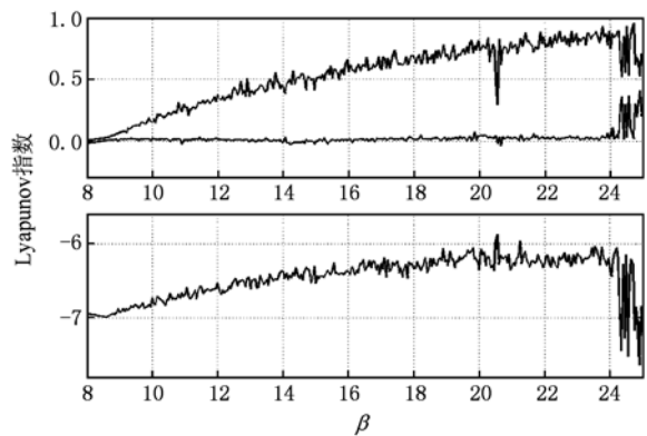
图 4 Lyapunov 指数谱, \alpha = 6, \gamma = 0.01, a = -3, b = 1, \beta \in [8, 25]
