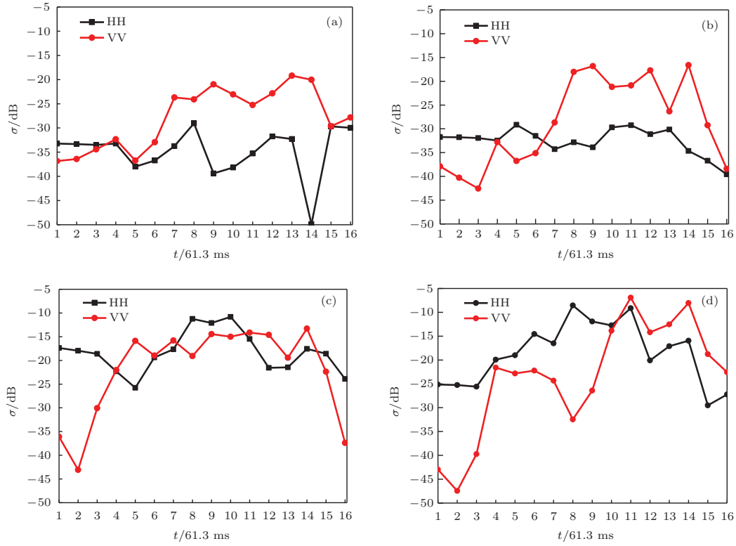
图3 不同入射角时卷曲中海浪后向电磁散射系数随时间的变化 (a) \theta_i = 45^\circ , u = 10 m/s; (b) \theta_i = 60^\circ , u = 10 m/s; (c) \theta_i = 85^\circ , u = 10 m/s; (d) \theta_i = 85^\circ , u = 15 m/s
