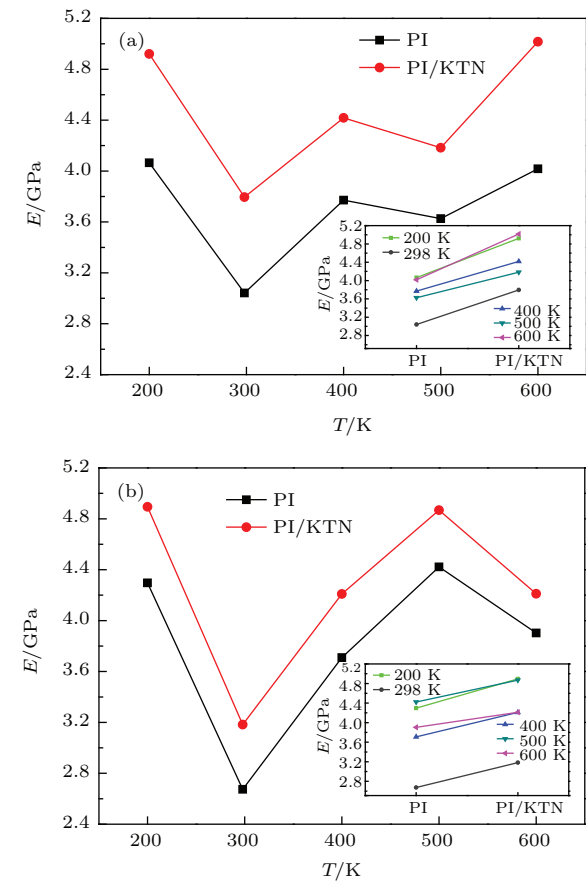
图2 不同压强和温度下PI和PI/KTN的杨氏模量(内插图为同一温度下PI和PI/KTN的杨氏模量) (a)压强为0 Pa; (b)压强为1 atm Fig. 2. The Young's modulus of PI and PI/KTN at different pressures and temperatures: (a) 0 Pa; (b) 1 atm. Inset shows the Young's modulus of PI and PI/KTN at the same temperature.
