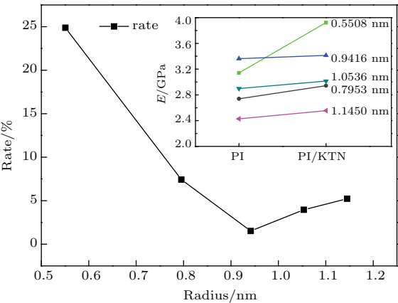
图3 杨氏模量增长率随纳米颗粒尺寸变化的规律 (内插图 为PI与PI/KTN的杨氏模量) Fig. 3. The growth rate of Young's modulus along with various sizes of nanoparticles (inset is the Young's modulus of PI and PI/KTN).
