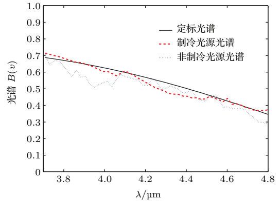
图 19 SiC 光源的光谱 Fig. 19. The recovered spectrum of the SiC light source.
