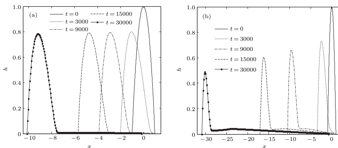
图 11 液滴演化历程 ( \Gamma = 0.02 ) (a) \Sigma_{ls} = \Sigma_{sg} = \Sigma_{lg} = 1.0 ; (b) \Sigma_{sg} = 1.01 , \Sigma_{ls} = \Sigma_{lg} = 1
