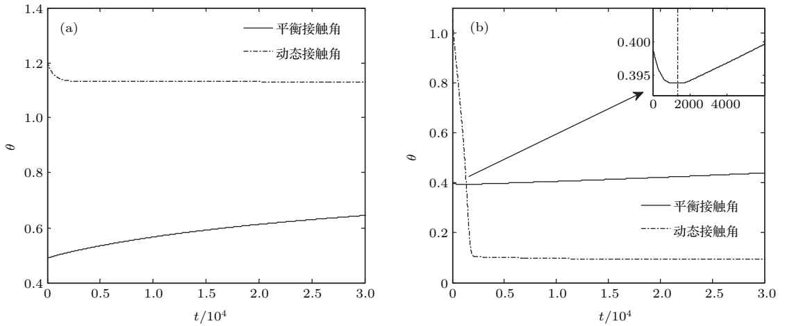
图 14 两侧接触角的变化 ( \Gamma = 0.02 , \Sigma_{lg} = 1.01 , \Sigma_{sg} = \Sigma_{ls} = 1.0 ) (a) 左侧接触角; (b) 右侧接触角 Fig. 14. Variation of contact angles on both sides of the droplet when \Gamma = 0.02 , and \Sigma_{lg} = 1.01 , \Sigma_{sg} = \Sigma_{ls} = 1.0 : (a) Left contact angles; (b) right contact angles.
