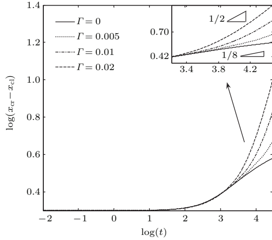
图4 温度梯度对铺展范围的影响 ( \Sigma_{sg} = \Sigma_{lg} = \Sigma_{ls} = 1.0 ) Fig. 4. Effect of temperature gradient on spreading range when \Sigma_{sg} = \Sigma_{lg} = \Sigma_{ls} = 1.0 .
