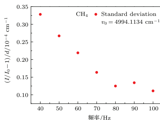
图 3 一倍标准偏差随扫描频率的变化 Fig. 3. Relationship of one standard deviation ( 1\sigma ) versus scanning frequency.
