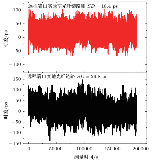
图 9 (网刊彩色) 实验室光纤与实地光纤链路时差变化测量结果 (红色曲线表示实验室光纤, 黑色曲线表示实地光纤) Fig. 9. (color online) The measured time interval variation results of the laboratory fiber link (red line) and the filed fiber link (black line).
