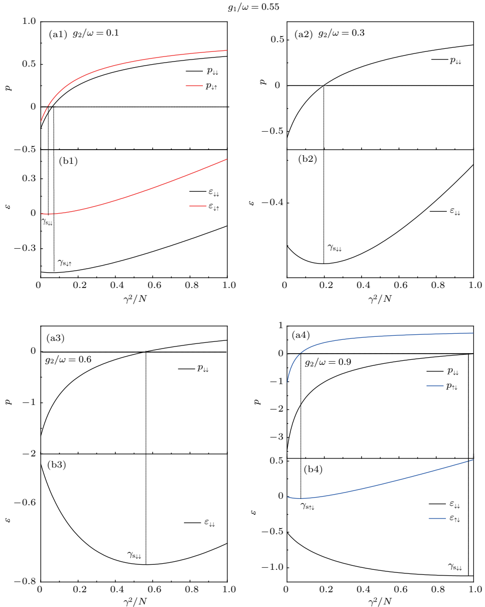
图2 极值方程 P_k(\gamma_{sk}) = 0 (a1)–(a4) 和平均能量曲线 \epsilon (b1)–(b4) 随平均光子数 \gamma^2/N 的变化 (给定的条件是: 第一组分原子与场的耦合强度为 g_1/\omega = 0.55 和 g_2/\omega = 0.1, 0.3, 0.6, 0.9 , 其中 k = \downarrow\downarrow (黑线), k = \downarrow\uparrow (红线), k = \uparrow\downarrow (蓝线)) Fig. 2. Graphical solutions of the extremum equation P_k(\gamma_{sk}) = 0 (a1)–(a4) and the corresponding average energy curves \epsilon (b1)–(b4) as the function of the mean photon number \gamma^2/N for k = \downarrow\downarrow (black line) and k = \downarrow\uparrow (red line) (or k = \uparrow\downarrow (blue line)). The plotted parameters are given by g_1/\omega = 0.55 and g_2/\omega = 0.1, 0.3, 0.6, 0.9 .
