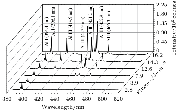
图2 在距离样品表面 0.65 mm 处, 激光作用后延迟 50 ns, 探测门宽 200 ns 下记录的等离子体发射光谱图(气压为 2.8 Pa) Fig. 2. Spectra of optical emission from the plasma recorded at a delay of 50 ns with a gate of 200 ns and at a distance of 0.65 mm from the sample surface(Background pressure was 2.8 Pa).
