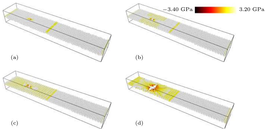
图 8 带孔洞的含孪晶界模型断裂前后应力分布状态 (a) \epsilon = 14.34\% ; (b) \epsilon = 16.92\% ; (c) \epsilon = 18.25\% ; (d) \epsilon = 20.87\% Fig. 8. Distribution of tensile stress in the voided mono-layer MoS 2 sheet with twin boundaries: (a) \epsilon = 14.34\% ; (b) \epsilon = 16.92\% ; (c) \epsilon = 18.25\% ; (d) \epsilon = 20.87\% .
