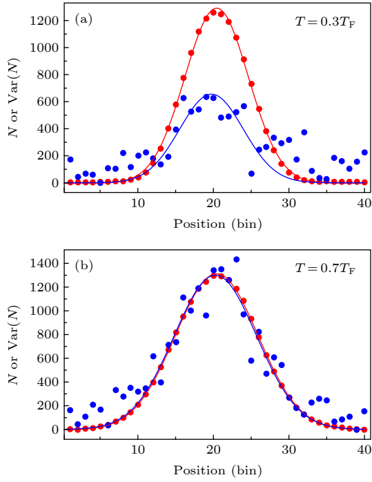
图 5 不同温度下原子密度与密度涨落的空间分布. 图中红线为原子密度分布, 蓝线为密度涨落分布 Fig. 5. Spatial distribution of atomic density and density fluctuation at different temperatures. The red line is the atomic density distribution and the blue line is the density fluctuation distribution.
