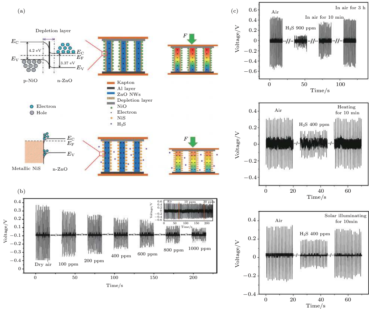
图 3 基于柔性 PENG 的自驱动 H_2S 气体传感器 [23] (a) 硫化反应的传感机制; (b) 响应过程; (c) 复原过程 Fig. 3. Self-driven H_2S gas sensor based on flexible PENG [23] : (a) The sensing mechanism of vulcanization reaction; (b) response process; (c) recovery process.
