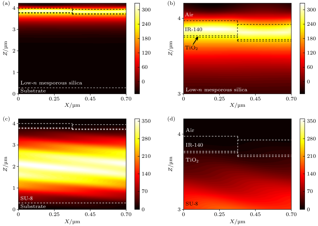
图3 TE偏振入射下共振波长处的电场强度 |E|^2 分布图: (a) 多孔二氧化硅结构和(b)局部放大图; (c) SU-8结构和(d)局部放大图 Fig. 3. Electric field intensities |E|^2 for the TE-polarized light incidence at resonance wavelength: (a) mesoporous silica structure and (b) partially enlarged view; (c) SU-8 structure and (d) partially enlarged view.
