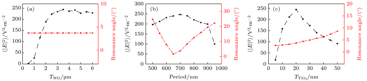
图4 增益介质区域的局域电场均方值 \langle |E|^2 \rangle 和共振角度随 (a) 多孔二氧化硅层厚度, (b) 光栅周期与(c) TiO 2 厚度的变化曲线 Fig. 4. Calculated \langle |E|^2 \rangle value and resonance angle versus (a) the thickness of the mesoporous silica, (b) the grating period and (c) the thickness of TiO 2 .
