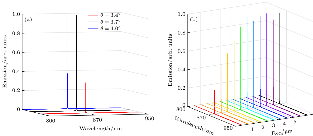
图 6 (a) 不同入射角下的激光出射谱线; (b) 3.7^\circ 共振条件时多孔二氧化硅层厚度与激光出射谱线的关系 Fig. 6. (a) Normalized emission spectra of the laser at different incident angles; (b) normalized emission spectra of the laser at the incident angle of 3.7^\circ vs. thickness of the mesoporous silica.
