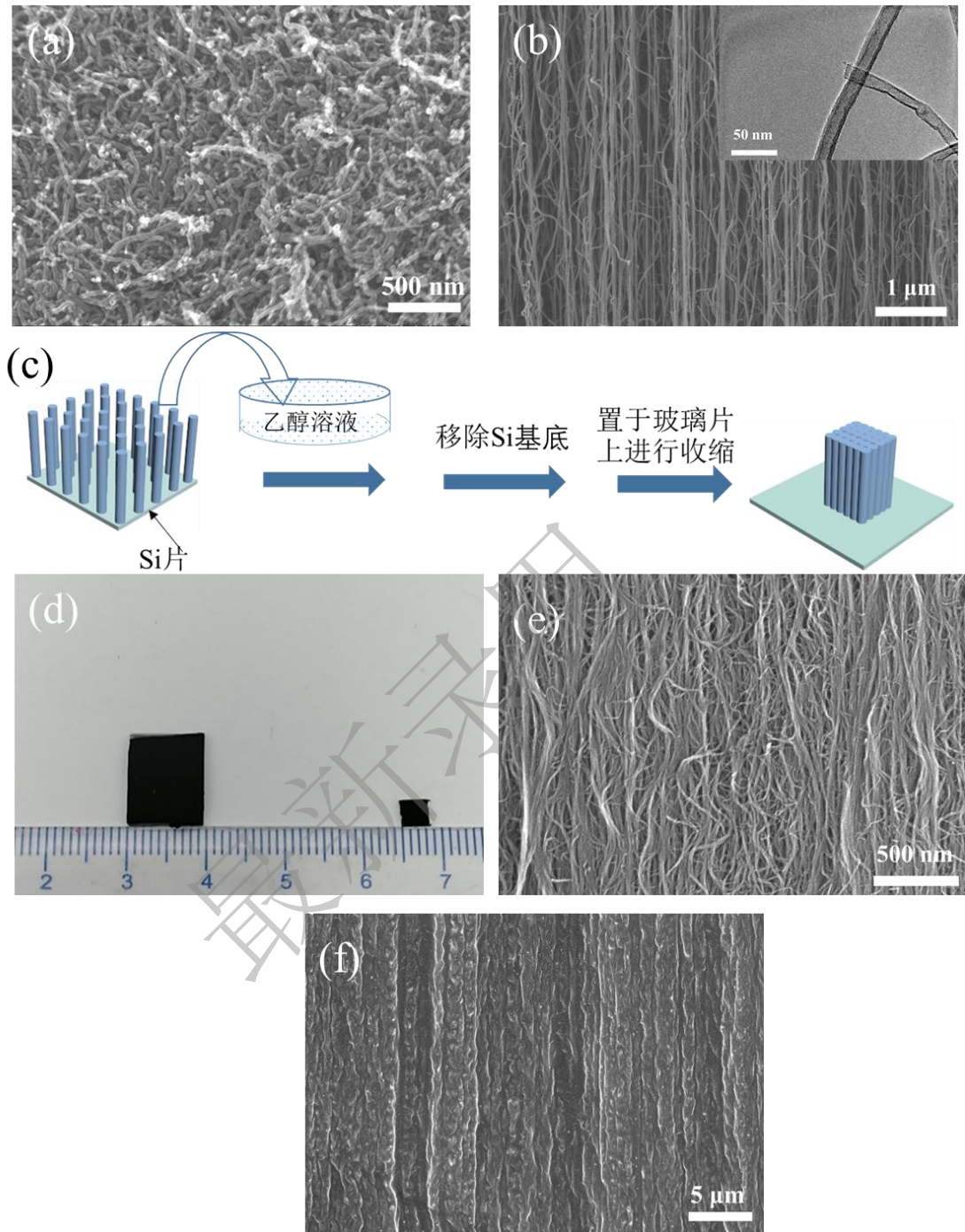
图2 扫描电子显微镜图：(a)商业无规碳管粉末；(b)取向碳纳米管阵列(内部插图为单根碳纳米管 TEM 图)；(c)高密度取向碳纳米管阵列制备过程图；(d)收缩前后阵列尺寸对比图；(e)高密度取向碳纳米管阵列 SEM 图；(f)凝胶包埋后 ACNT@PVA@HQ 复合膜 SEM 图。 Figure 2. The image of scanning electron microscope(SEM): (a) CCNT; (b)ACNT(insert: The TEM image of ACNT); (c)Preparation process of the highly densified carbon nanotube arrays(DACNT); (d) Comparison of the arrays before and after shrinkage; (e) The SEM image of DACNT; (f)The SEM image of the ACNT@PVA@HQ composite device
