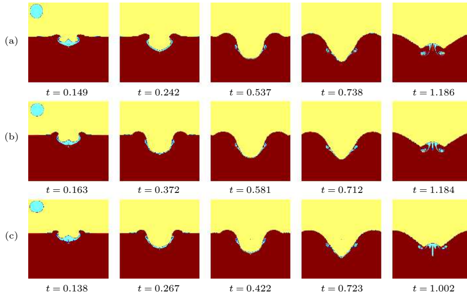
图 5 不同工况下自由液面随时间的运动过程 ( Fr = 75 , We = 64.4 , Re = 1160 , V_i = 4 m/s) (a) AR = 1.16 ; (b) AR = 1.00 ; (c) AR = 0.84
