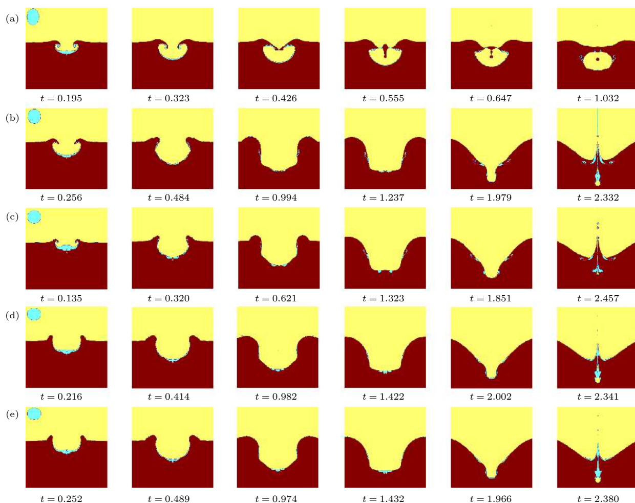
图 6 不同工况下自由液面随时间的运动过程 ( Fr = 112.5 , We = 145 , Re = 1740 , V_i = 6 m/s) (a) AR = 1.33 ; (b) AR = 1.16 ; (c) AR = 1.00 ; (d) AR = 0.84 ; (e) AR = 0.67
