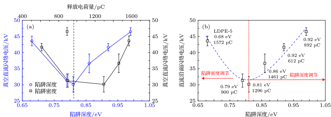
图9 陷阱参数与真空沿面闪络电压之间的关系 (a) 陷阱深度、陷阱密度与闪络电压的关系; (b) 陷阱对直流闪络电压的影响 Fig. 9. Relationship between trap parameters and surface flashover performance: (a) Trap depth, trap density and surface flashover voltage; (b) trap and surface flashover voltage.
