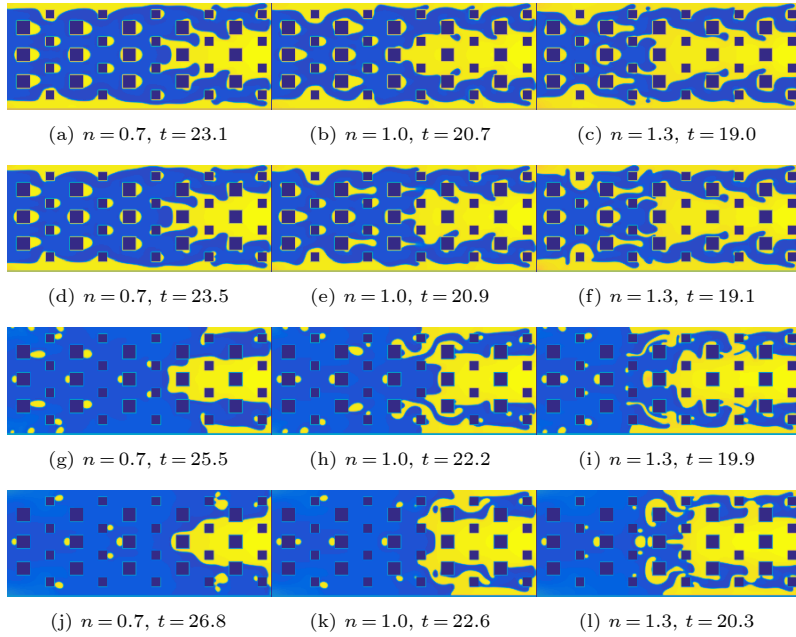
图 13 不同的润湿性角度 \theta 下, 被驱替液为剪切变稀、牛顿与剪切变稠流体时得到的指进形态图 (a)–(c) \theta = 45^\circ ; (d)–(f) \theta = 60^\circ ; (g)–(i) \theta = 120^\circ ; (j)–(l) \theta = 135^\circ Fig. 13. Final finger patterns obtained under different values of contact angles \theta for shear thinning, Newtonian and shear thickening fluids: (a)–(c) \theta = 45^\circ ; (d)–(f) \theta = 60^\circ ; (g)–(i) \theta = 120^\circ ; (j)–(l) \theta = 135^\circ .
