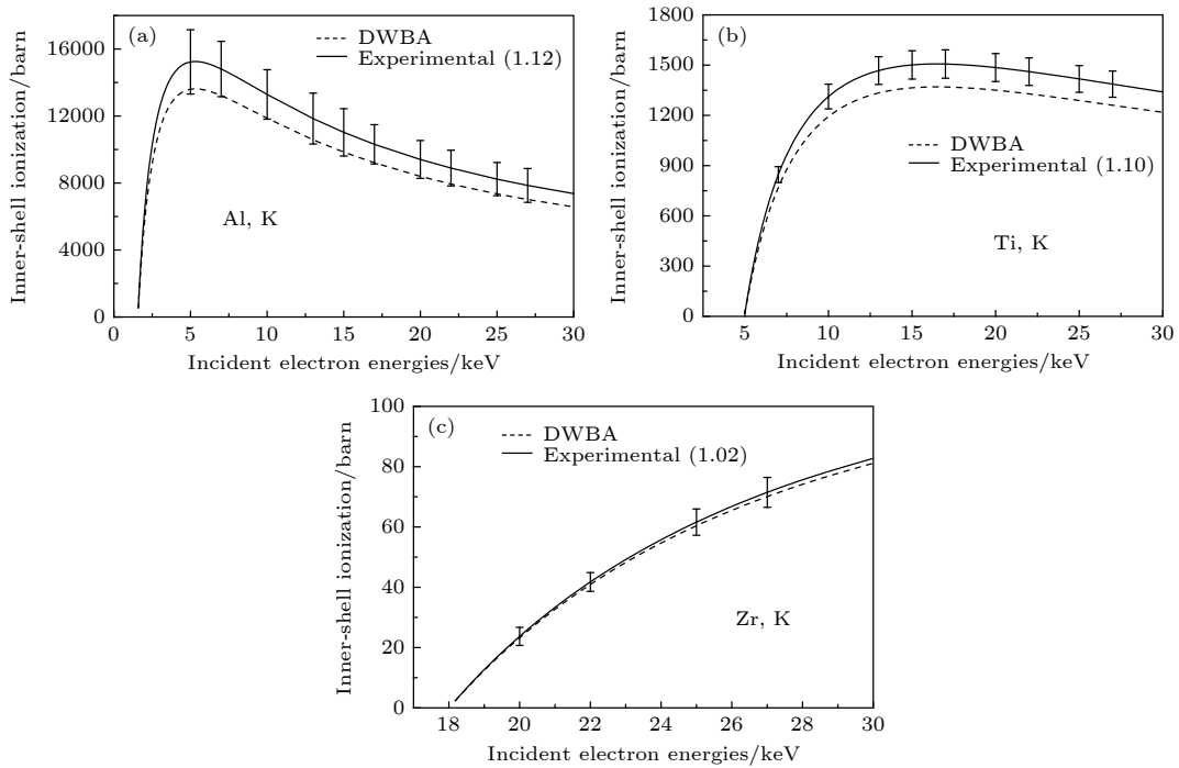
图 8 (a) Al, (b) Ti, (c) Zr 元素实验 K 壳电离截面 (实线) 与 DWBA 理论值 (虚线), 括号内为修正系数 Fig. 8. Experimental K-shell ionization cross sections of (a) Al, (b) Ti, (c) Zr (solid lines) and the DWBA theoretical values (dashed lines). The scaling factors are given in parentheses.
