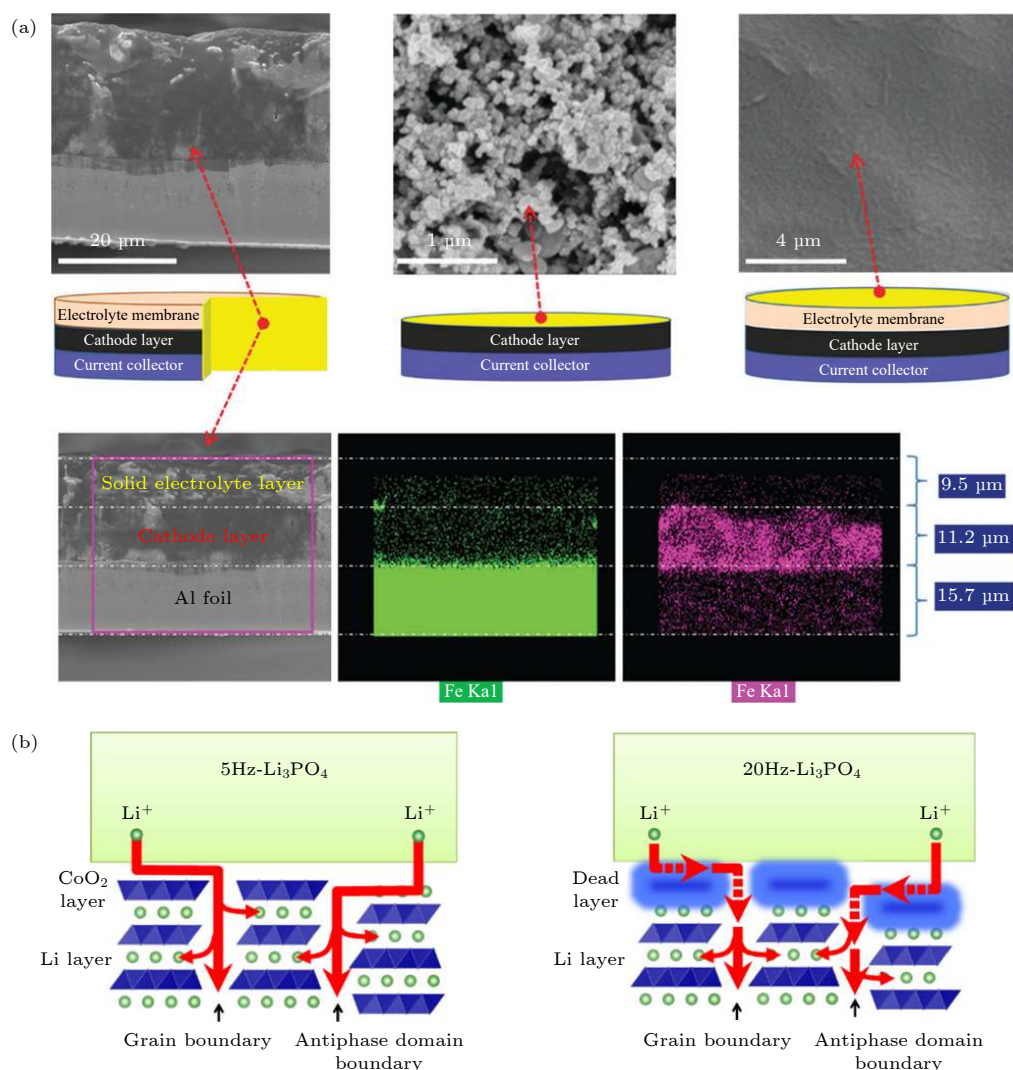
图 4 改善固-固界面物理接触 (a) 阴极支撑的固态电解质方案 [18] ; (b) 电极表面原子尺度结构调控全固态电池的界面 [19] Fig. 4. Improvement of the physical contact of the solid-solid interface: (a) A cathode-supported solid electrolyte membrane framework [18] ; (b) the surface structure of the electrode controlled by the interface of the all-solid-state battery [19] .
