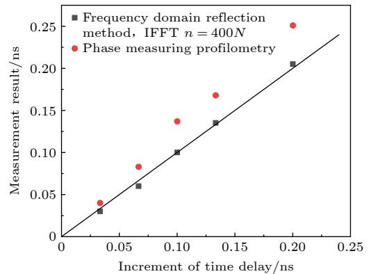
图 6 频域反射法与相位法对参考延时测量结果的比较 Fig. 6. Comparison of measurement results between frequency domain reflection method and phase measuring profilometry.
