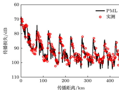
图 1 200 Hz 时声压传播损失曲线与实验数据对比图 [26] Fig. 1. Comparison diagram of transmission loss and experimental data at 200 Hz [26] .
