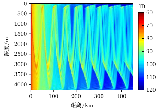
图 3 频率平均传播损失伪彩图 Fig. 3. Pseudo color map of transmission loss with frequency averaged.
