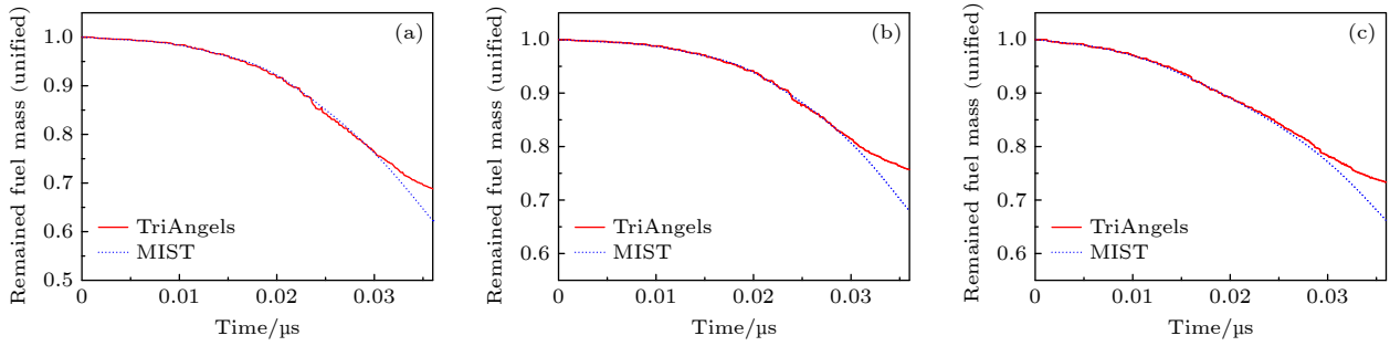
图 6 不同初始条件影响下 MIST 与 TriAngels 计算得到的套筒内剩余燃料质量随时间演化关系 ( A = 0.31 ) (a) h = 0.75 cm; (b) g = 2 mg/cm 3 ; (c) r_{LEH} = 0.15 cm Fig. 6. Comparison between remained fuel mass calculated by MIST and TriAngels under different initial parameters ( A = 0.31 ): (a) h = 0.75 cm; (b) g = 2 mg/cm 3 ; (c) r_{LEH} = 0.15 cm.
