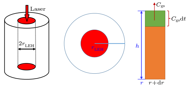
图 2 端面效应简化模型示意图 Fig. 2. Schematic of simplified model describing end loss effect.
