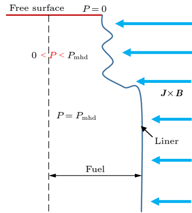
图 3 由轴向压力不平衡引发的腊肠不稳定性种子示意图 Fig. 3. Schematic of instability seed caused by axial pressure imbalance.
