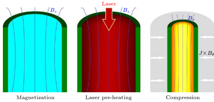
图 1 MagLIF 过程示意图 (包含 3 个主要阶段) Fig. 1. Schematic of MagLIF process, including three main stages.
