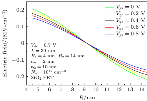
图 9 不同栅电压下电场沿半径的分布 Fig. 9. Electric field distribution along the radius with different gate voltage.
