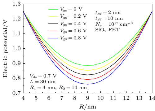
图 8 不同栅电压下电势沿半径的分布 Fig. 8. Electric potential distribution along the radius with different gate voltage.
