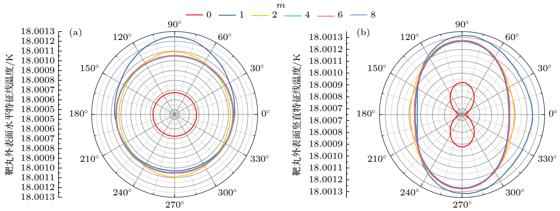
图 8 靶丸外表面特征线温度分布 (a)靶丸外表面水平特征线温度分布曲线; (b)靶丸外表面竖直特征线温度分布曲线 Fig. 8. Temperature distribution of characteristic line of capsule outside surface: (a)Horizontal characteristic line; (b) vertical characteristic line.
