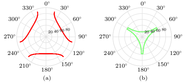
图8 (a)镀金属膜与(b)无镀膜角锥棱镜( n \approx 1.44@1550\text{ nm} )的高反射率入射方向范围 Fig. 8. High optical efficiency incidence direction range of (a) metal-coated and (b) uncoated CCR ( n \approx 1.44@1550\text{ nm} ).
