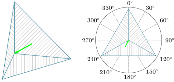
图6 金属膜角锥棱镜满足高效率后向反射的折射光线矢量 Fig. 6. High efficiency backward reflection ray vector in metal-coated CCR.
