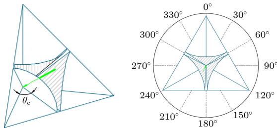
图7 无镀膜角锥棱镜满足高效率后向反射的折射光线矢量 Fig. 7. High efficiency backward reflection ray vector in uncoated CCR.
