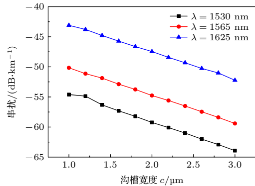
图 8 沟槽宽度 c 的变化对 LP 31 芯间串扰的影响 Fig. 8. The influence of the change of trench width c on the inter-core crosstalk of LP 31 mode.
