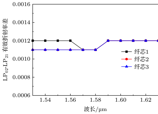
图 6 3种纤芯中 LP 02 与 LP 21 模的有效折射率差 Fig. 6. The refractive index difference between LP 02 and LP 21 modes in the three cores.
