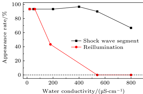
图 5 各种水电导率下流光丝的再发光和冲击波串分段出现频度 Fig. 5. Appearance rate of the re-illumination and segmentation in shockwave pattern of the streamer filament at different water conductivity.
