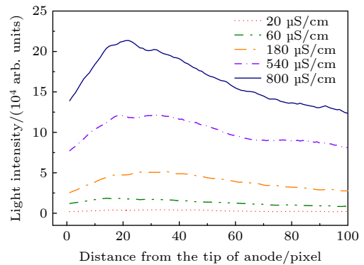
图 7 不同水电导率下流光丝轴向光强分布 Fig. 7. Axial distribution of light intensity of the streamer filament at different water conductivity.
