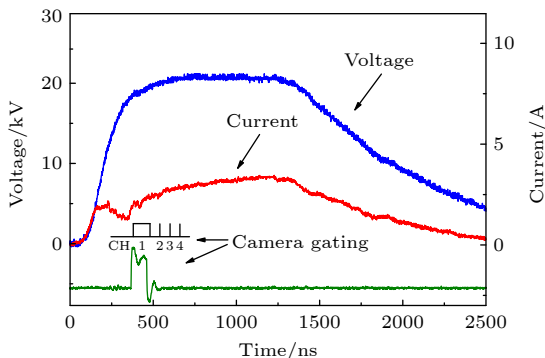
图 2 180 \mu\text{S}/\text{cm} 水电导率下的放电电压和电流波形以及相机快门信号 Fig. 2. Waveforms of the discharge voltage and current at water conductivity of 180 \mu\text{S}/\text{cm} , as well as the camera gating signal.
