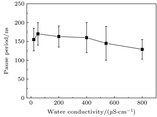
图 6 不同水电导率条件下流光丝的暂停时间 Fig. 6. The pause period of the streamer filament at different water conductivity.
