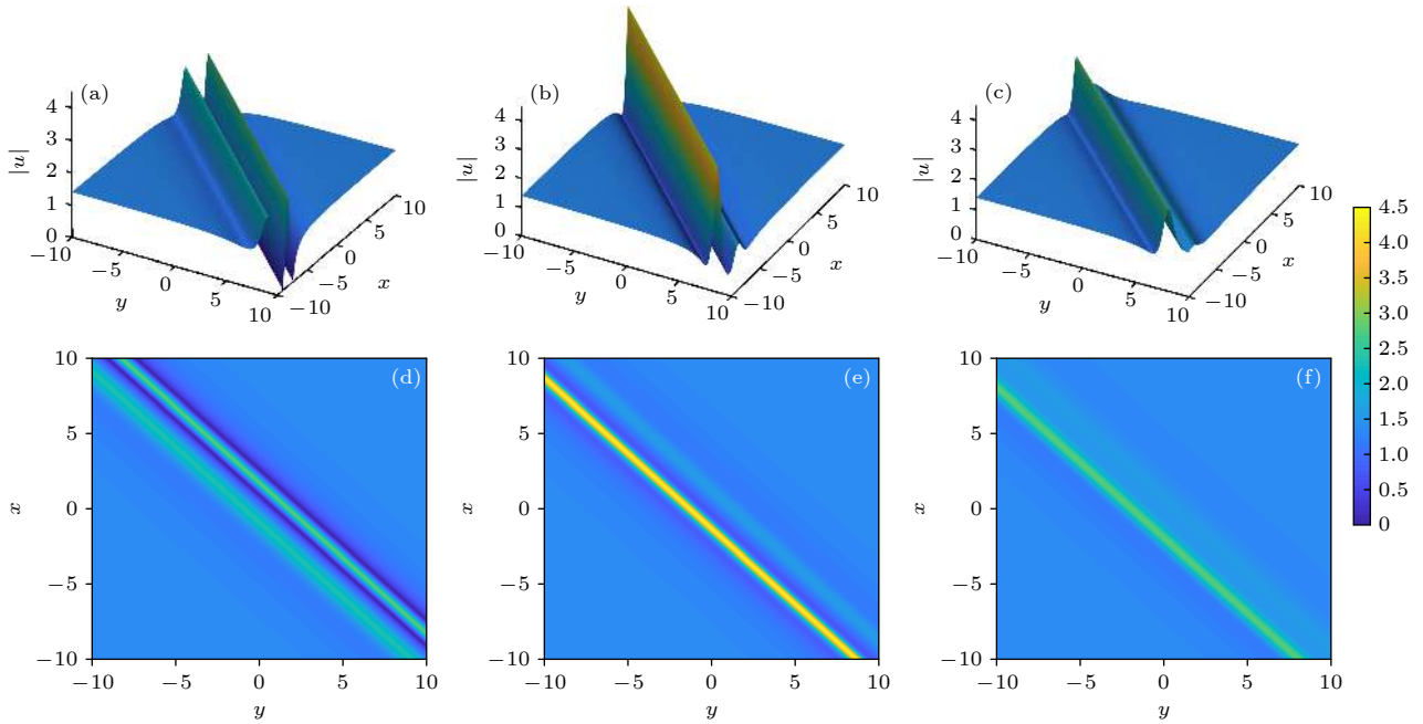
图 5 传播距离 z = 0, 0.5, 1.0 时二阶线怪波簇 |u| (a), (b), (c) 三维图; (d), (e), (f) 对应 x-y 面上的投影图; (a), (d) A = 2.76 ; (b), (e) A = 4.36 ; (c), (f) A = 2.78 ; 参数 w_0 = \gamma = \beta_0 = 1, \varsigma_0 = \zeta_0 = \varphi_0 = 0, \mu = 40, \delta = 20
