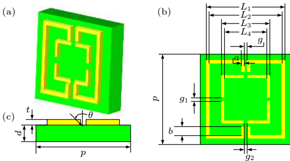
图 1 双明模耦合的单元结构图 (a) 由顶层金属层和底层非金属层构成的超材料结构的三维视图; (b) 所设计超材料结构的正视图; (c) 所设计超材料的侧视图 Fig. 1. Unit structure diagram of bright-bright mode coupling: (a) 3D view of metamaterial structure consisting of top metal layer and bottom nonmetal layer; (b) view of the designed metamaterial structure; (c) side view of the designed metamaterial structure.
