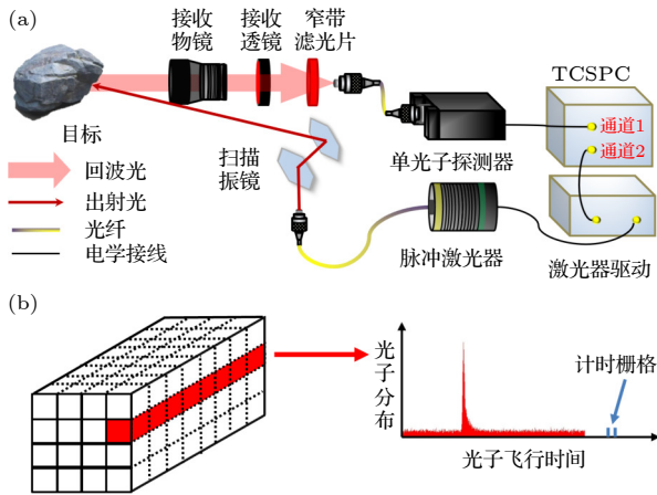
图 1 光子计数激光雷达原理图 (a) 成像系统示意图; (b) 三维回波示意图 Fig. 1. The schematic diagram of photon counting LiDAR: (a) Description of the imaging system; (b) description of the three dimensional echo.
