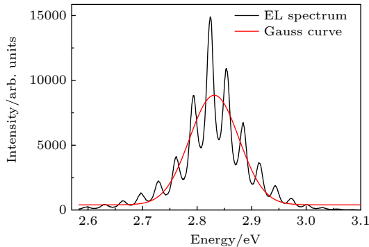
图 5 蒸镀顶部反射镜前在垂直发光面方向测试的器件电致发光光谱(黑色线)及其 Gauss 拟合曲线(红色线) Fig. 5. Electroluminescence spectrum (black line) and its Gaussian fitting curve (red line) of the device without top DBR measured perpendicular to the light-emitting surface.
