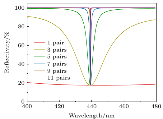
图 4 滤波器结构 DBR 的反射率模拟曲线 Fig. 4. Simulated reflectivity spectra of Ta 2 O 5 /SiO 2 DBR with filter structure.
