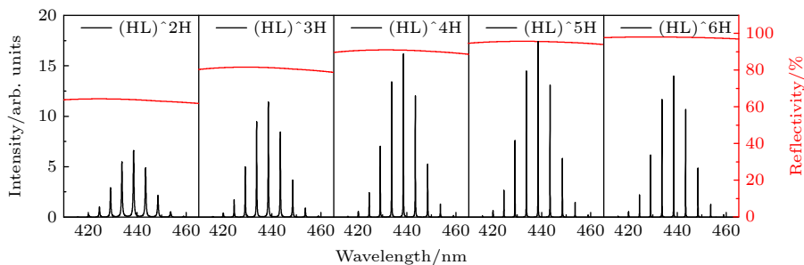
图 6 顶部蒸镀不同对数高反膜结构 DBR 时 RCLED 的模拟输出光谱(黑色线)和对应的顶部反射镜反射率模拟曲线(红色线) Fig. 6. Simulated electroluminescence spectra (black line) of RCLEDs and reflectivity spectra (red line) of the DBRs with high-reflective-film structure.
