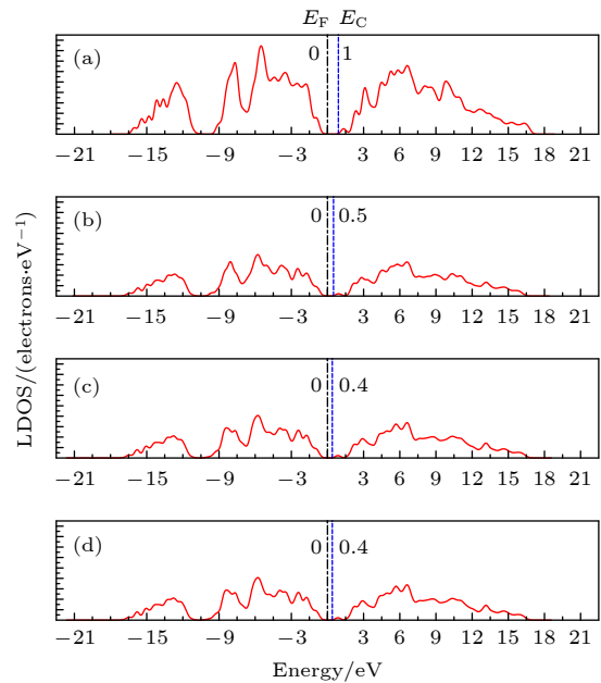
图 5 Cu(111)/SiC 体系在 SiC 区域的局域态密度图 (a) Cu/SiC; (b) Cu/1GR/SiC; (c) Cu/2GR/SiC; (d) Cu/3GR/SiC Fig. 5. Local density of states of SiC region for (a) Cu/SiC, (b) Cu/1GR/SiC, (c) Cu/2GR/SiC, and (d) Cu/3GR/SiC systems.
