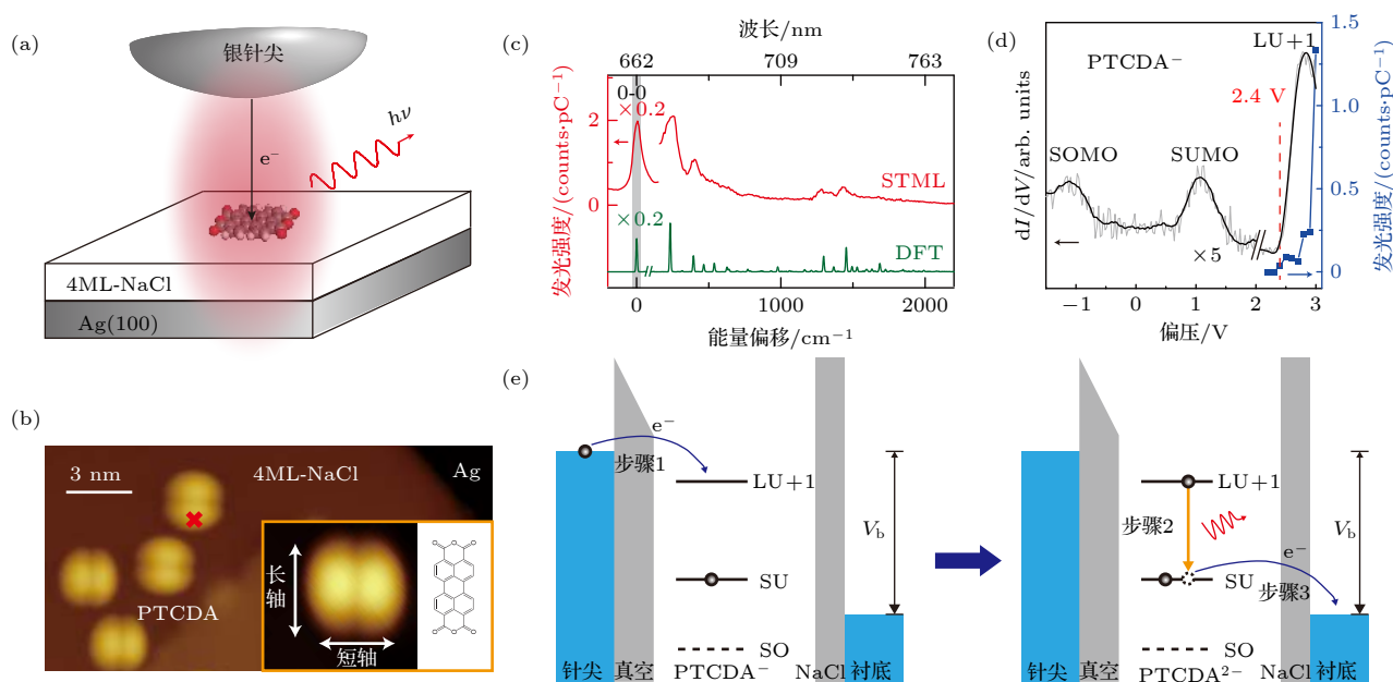
图 1 具有振动分辨的单个 PTCDA 分子瞬时 -2 价的电致发光 (a) 利用 STML 技术研究 PTCDA 分子电致荧光的实验示意图; (b) 吸附在 4 ML-NaCl/Ag(100) 表面 PTCDA 分子的 STM 扫描图像, 扫描条件为 1 V, 2 pA; 插图为单个 PTCDA 分子的 STM 扫描图像与对应取向的分子结构示意图; 比例尺为 3 nm; (c) 红色曲线对应在图 (b) 中红色 “ \times ” 处激发时获得的 STML 光谱 (+3 V, 50 pA, 60 s), 绿色曲线为 DFT 理论计算的单个 -2 价 PTCDA 分子的荧光光谱; (d) 黑色曲线对应在图 (b) 中红色 “ \times ” 处测量的 dI/dV 谱 ( -3 V, 40 pA), 蓝色点线为不同偏压下分子 STML 发光强度统计; (e) 瞬时 -2 价 PTCDA 分子的 STML 发光机制示意图 Fig. 1. Vibronically resolved electroluminescence from a single transient doubly charged PTCDA molecule. (a) Schematic of the STML experiment on a single PTCDA molecule on 4 ML-NaCl/Ag(100). (b) STM image of isolated PTCDA molecules adsorbed on 4 ML-NaCl/Ag(100) (+1 V, 2 pA), with the molecular structure given in the inset showing molecular orientation corresponding to the inset STM image. (c) Typical STML spectrum (+3 V, 50 pA, 60 s) (red curve) acquired at the red “ \times ” marked in (b). A DFT simulated fluorescence spectrum from a single doubly charged PTCDA molecule is also plotted for comparison (green curve). (d) Typical dI/dV spectrum (black curve) acquired at the red “ \times ” marked in (b). The setpoint for the dI/dV measurement was -3 V and 40 pA. The molecular emission intensities at different excitation voltages are also shown (blue filled rectangles). (e) Schematic of the mechanism for the molecular electroluminescence of PTCDA ^{2-} .
