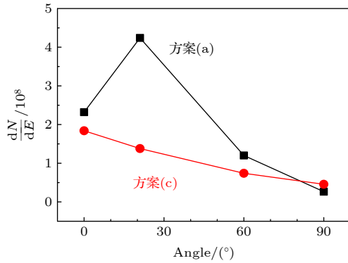
图 12 方案 (a) 与方案 (c) 的伽马射线能谱空间分布对比 Fig. 12. Comparison of spatial distributions of gamma-ray energy spectra between scheme-(a) and scheme-(c).
