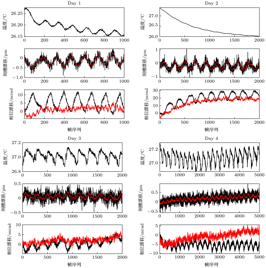
图 4 对热稳定测试数据进行像面漂移监测的结果示意. 刻槽漂移中, 黑色曲线代表原始检测结果, 红色曲线代表平滑得到的趋势线; 相位漂移中, 黑色曲线代表原始的相位漂移, 红色曲线代表校正后的相位漂移 Fig. 4. Schematic diagram of image plane drift monitoring results of thermal stability test data. In the graph of notch drift, the black curve represents the original result, and the red curve represents the smoothed trend line. In the graph of phase drift, the black curve represents the original result, and the red curve represents the corrected phase.
