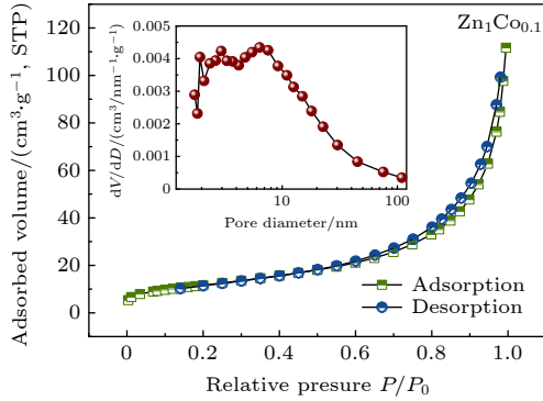
图 3 Zn 1 Co 0.1 复合微结构的氮吸附-脱附等温曲线与孔径分布曲线(插图) Fig. 3. Nitrogen adsorption-desorption isotherm and pore size distribution curve (inset) of Zn 1 Co 0.1 composite microstructure.
