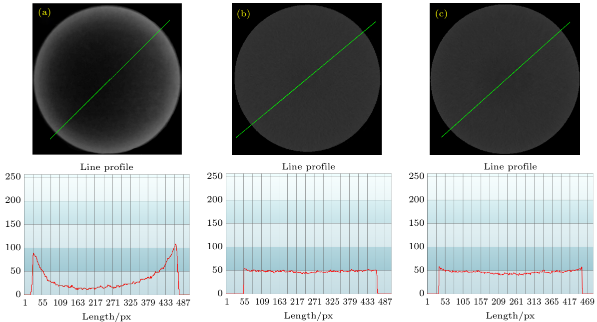
图 8 水模的均匀性响应 (a) 不使用 PFXRL, 重建的水模中平横断面图像及绿线对应的 CT 值; (b) 使用 PFXRL, 重建的水模中平横断面图像及绿线对应的 CT 值; (c) 采用 0.5 mm 厚的铝片附加滤过, 重建的水模中平横断面图像及绿线对应的 CT 值. 空气和水的 CT 值分别归一化为 0 和 50 Fig. 8. Uniformity response of the water phantom: (a) Reconstructed transaxial image of the uniformity phantom without using PFXRL and radial signal profile taken from the green line; (b) reconstructed transaxial image of the uniformity phantom with using PFXRL and radial signal profile taken from the green line; (c) reconstructed transaxial image of the uniformity phantom with a 0.5 mm thick aluminum sheet as filter and radial signal profile taken from the green line. The CT values of air and water are normalized to 0 and 50, respectively.
