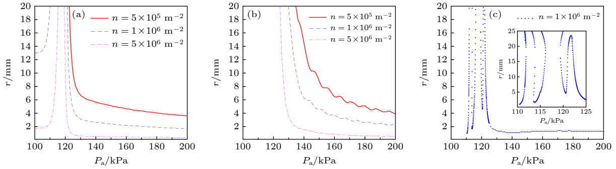
图 4 不同气泡半径时, 气泡数密度对气泡链半径随声压演变规律的影响, 声波频率 f = 20\text{kHz} (a) R_{10} = R_{20} = 3\ \mu\text{m} , (b) R_{10} = 5\ \mu\text{m} , R_{20} = 3\ \mu\text{m} , (c) R_{10} = 3\ \mu\text{m} , R_{20} = 5\ \mu\text{m}
