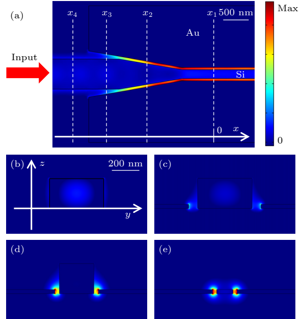
图 2 硅基混合表面等离子激元光场窄化器件 ( W_{Si} = 120 nm, g = 30 nm, h_m = 30 nm) 的光场分布图 (a) 整体俯视图; (b)–(e) 对应于 x_1 = 0 \mu m, x_2 = -0.8 \mu m, x_3 = -1.4 \mu m, x_4 = -2 \mu m 的截面图 Fig. 2. Optical field distribution of the silicon hybrid plasmonic nanofocusing device ( g = 30 nm, W_{Si} = 450 nm, h_m = 30 nm): (a) Overall top view; (b)–(e) cross-sectional view corresponding to x_1 = 0 \mu m, x_2 = -0.8 \mu m, x_3 = -1.4 \mu m, x_4 = -2 \mu m.
