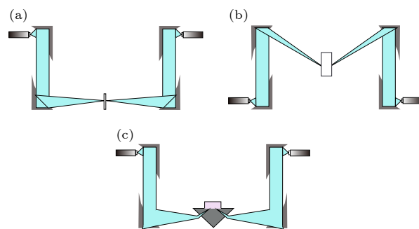
图 3 太赫兹光谱检测技术 (a) 透射式太赫兹光谱系统; (b) 反射式太赫兹光谱系统; (c) 衰减全反射太赫兹光谱系统 Fig. 3. Terahertz spectral detection technology: (a) Transmitted THz spectral system; (b) reflected THz spectral system; (c) attenuated total reflection THz spectral system.
