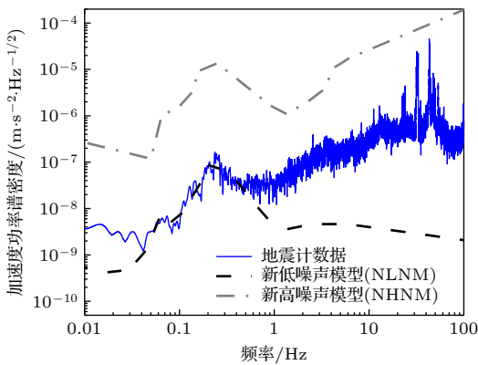
图 10 测试地点的地面振动加速度功率谱密度 Fig. 10. The power spectrum density of the ground vibration acceleration at the measurement site.
