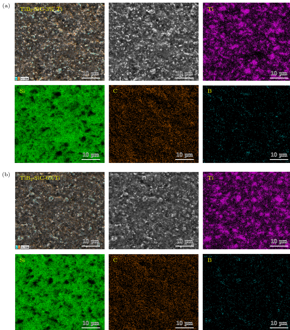
图 2 (a) TiB 2 -SiC-Ti(Ti 的质量分数为 3%) 样品和 (b) TiB 2 -SiC-Ti(Ti 的质量分数为 6%) 样品的能量色散 X 射线光谱图 Fig. 2. Energy dispersion X-ray spectroscopy of TiB 2 -SiC-Ti (the mass fraction of Ti is 3%) samples (a) and TiB 2 -SiC-Ti (the mass fraction of Ti is 6%) samples (b).
