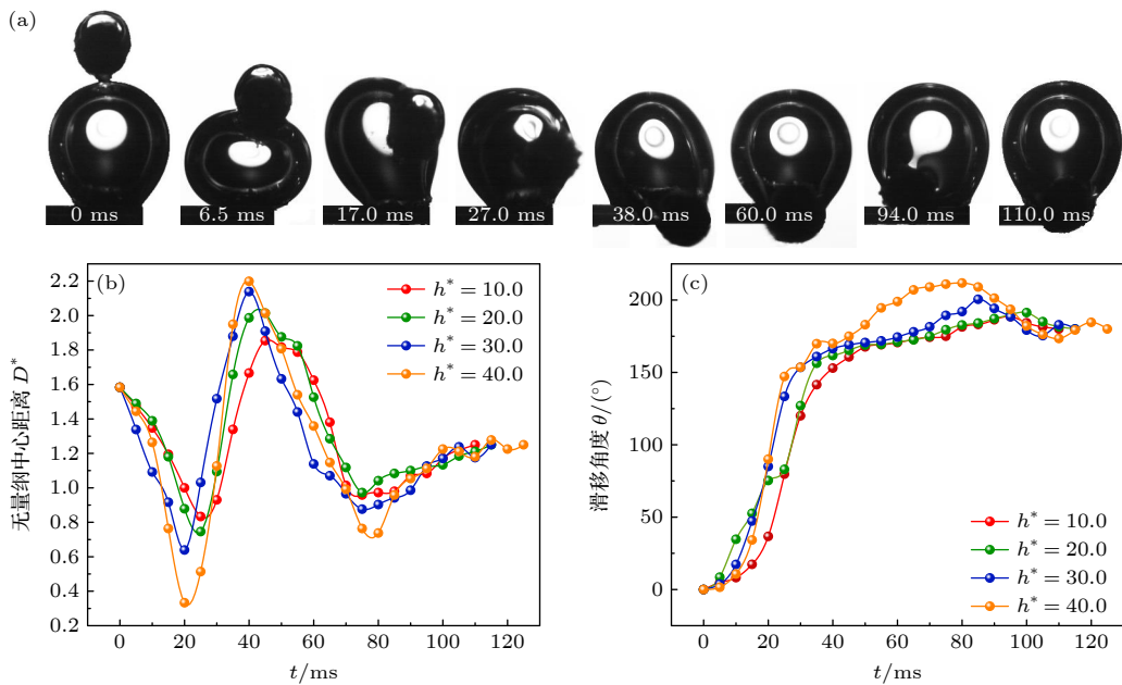
图 6 Janus 颗粒撞击气泡的动态过程及曲线图 (a) 动态过程图 ( h^* = 10.0 ); (b) D^* 随时间 t 变化的曲线图; (c) \theta 随 t 变化的曲线图 Fig. 6. Dynamic process and curve of Janus particle impacting bubble: (a) Dynamic process ( h^* = 10.0 ); (b) process curves for D^* changing with t ; (c) process curves for \theta changing with t .
