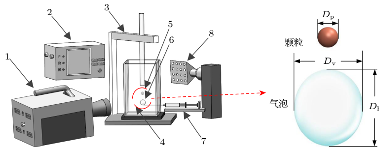
图 3 实验装置图 (1, 高速摄影仪; 2, 数据采集仪; 3, xyz 三轴微位移平台; 4, 亚克力玻璃池; 5, 实验样品; 6, 气泡; 7, 高精度注射器; 8, LED 背光灯) Fig. 3. Diagram of the experimental device. 1, high-speed camera; 2, data collector; 3, xyz three-axes micro-displacement platform; 4, acrylic glass cell; 5, experimental sample; 6, bubble; 7, high-precision syringe; 8, LED backlight.
