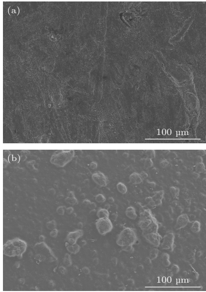
图 2 Janus 颗粒表面 SEM 图 (a) 亲水侧表面; (b) 超疏水侧表面 Fig. 2. SEM images of Janus particle surface: (a) Hydrophilic side surface; (b) superhydrophobic side surface.
