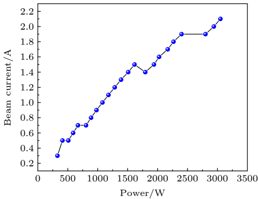
图 9 离子束电流随功率变化曲线 Fig. 9. Ion beam current as a function of input power.
