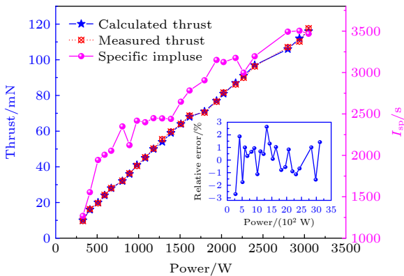
图 10 推力、比冲随功率变化曲线 Fig. 10. Thrust, specific impulse as a function of input power.
