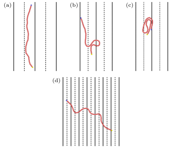
图 12 半刚性链在不同区域宽度下的构象快照 (a) d = 8 , 非活性区的沿 y 方向伸展状态; (b), (c) d = 6 , 跨区域的屈曲和屈曲折叠构象; (d) d = 3 , 跨越多个区域的蛇行构象 Fig. 12. Snapshots of the conformation of semi-rigid chains at different domain widths: (a) d = 8 , stretching along the y -direction in the inactive region; (b), (c) d = 6 , buckling and buckling-folded conformation across regions; (d) d = 3 , serpentine conformation spanning multiple regions.
