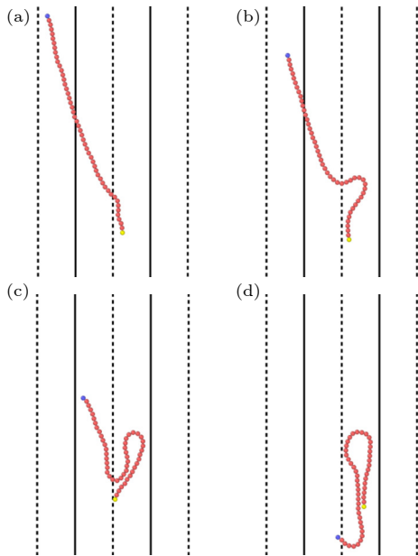
图 11 半刚性链跨区域运动的快照 ( d = 8 ), 头部从非活性区进入活性区失去自驱力, 链段往前推挤形成屈曲拱起 Fig. 11. Snapshot of the across region motion of the semi-rigid chain ( d = 8 ). The head enters the active region from passive and loses self-propelled force, and the chain segment is pushed forward to form buckling.
