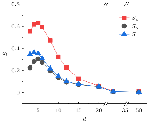
图 10 柔性链的向列序参数 S 与区域宽度 d 的非单调性变化关系, 在 d = 5 左右存在峰值, S_a 相对变化较大 Fig. 10. Nonmonotonic relationship of the nematic order parameter S and the region width d of the flexible chain. There is a peak around d = 5 , and the change of S_a is large relatively.
