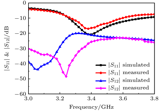
图 9 圆形阵列天线阵元反射系数模和相邻阵元间隔高度 Fig. 9. Element reflection and adjacent isolation of the circular array.
