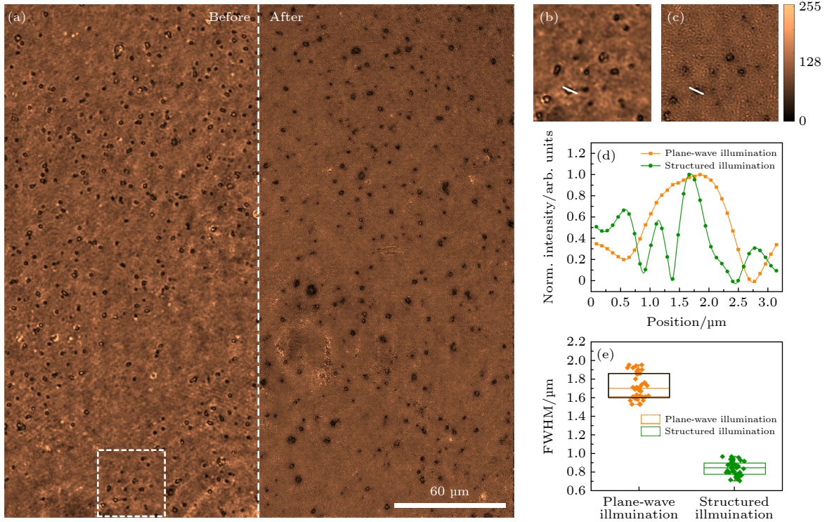
图 4 基于平行光/结构光照明数字全息显微对二氧化硅小球的成像结果 (a) 平行光(左)和结构光(右)照明时 DHM 获得的振幅图像; (b) 和 (c) 图 (a) 中白色方框区域在使用平行光照明和结构光照明的重构结果; (d) 图 (b) 和 (c) 中沿白色虚线的强度分布; (e) 平行光/结构光照明 DHM 的空间分辨率比较, 在图 (a) 中随机选择 35 个小球, 并对其在两个成像模式下半高全宽进行统计 Fig. 4. Plane-wave/structured-illumination based DHM imaging of SiO 2 beads: (a) Images of SiO 2 beads obtained by DHM with parallel illumination and structure illumination, respectively; (b) and (c) the magnified images within the white-box area in panel (a) obtained by plane-wave and structured illumination based DHM, respectively; (d) the intensity distributions along the white lines in panel (b) and (c); (e) statistics of lateral resolution of the two imaging modalities by randomly choosing and FWHM analysis of 35 beads for in panel (a).
