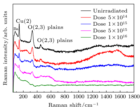
图6 不同剂量 H^+ 离子辐照前后样品的拉曼光谱 Fig. 6. Raman spectra of samples before and after H^+ ion irradiation with different doses.
