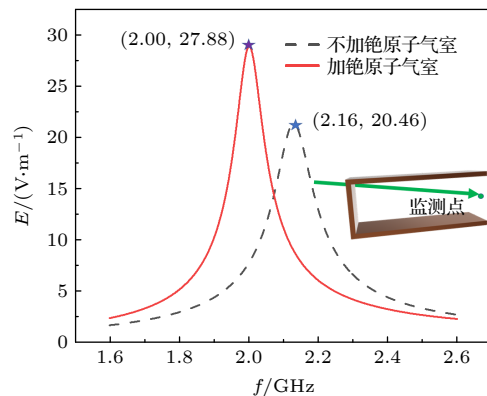
图 2 观测点电场强度随频率的变化 Fig. 2. Variation of electric field intensity at observation point with frequency.
