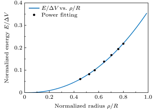
图 13 成像径向位置与离子能量的拟合关系曲线 Fig. 13. Normalized curve of imaging radial position and ion energy.
